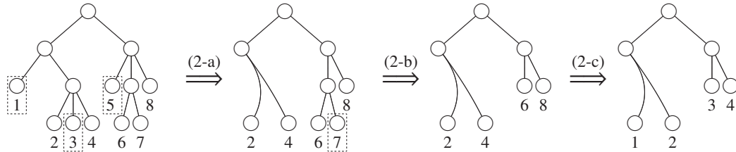
Figure 2: A behavior of Procedure 1: It describes an iteration of Steps (2a)–(2c): the dashed box specifies the leaves to which contraction operations are applied to at the step.
