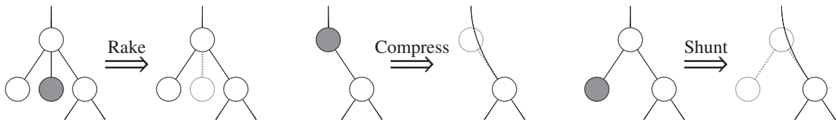
Figure 1: Primitive contraction operations applied to the gray-colored nodes: Rake (left), Compress (middle), and Shunt (right).
