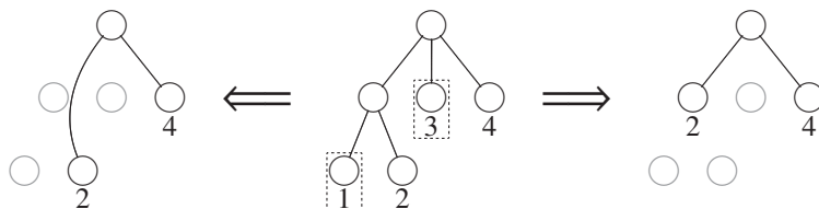
Figure 3: Critical applications of primitive contraction operations: the left describe the case where Shunt-L removes the parent, and the right describes the case where Shunt-L removes the sibling.
