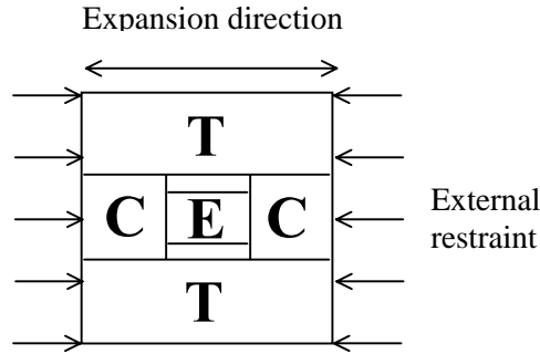
Fig.-1.4 Equivalent one-dimensional composite model of expansive concrete
