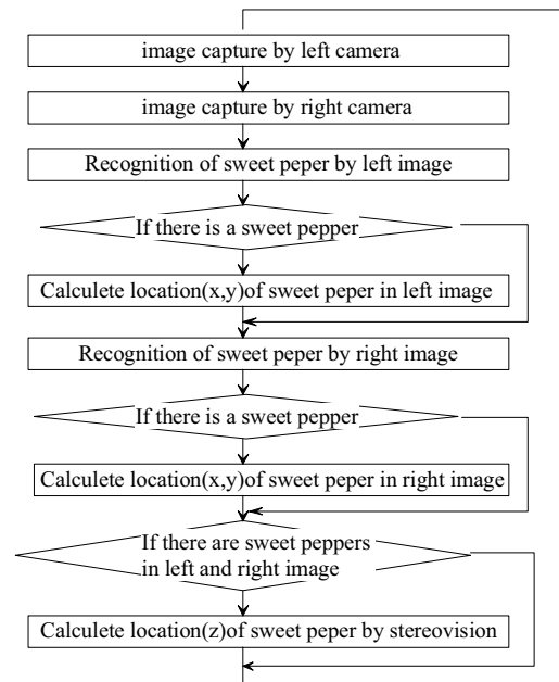
Fig.10 flow chart of image possessing
