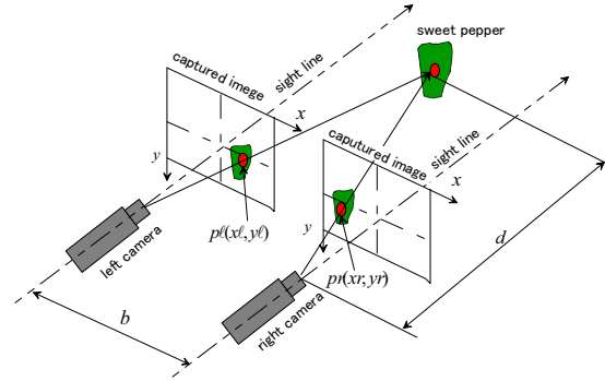
Fig.9 Parallel stereovision
