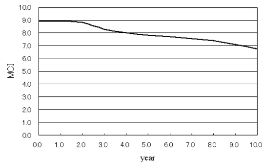
Figure 11. MCI deterioration forecast
