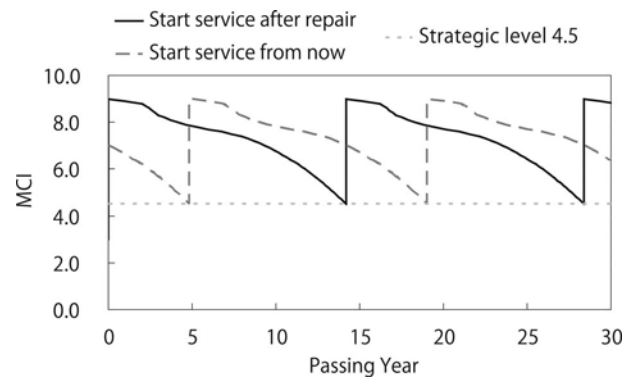
Figure 12. Degradation of MCI by passing year and recovery by repair
