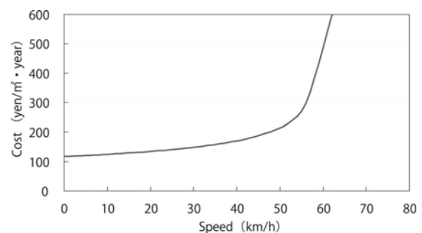
Figure 13. Supply function
