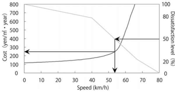
Figure 14. Equilibrium analysis
