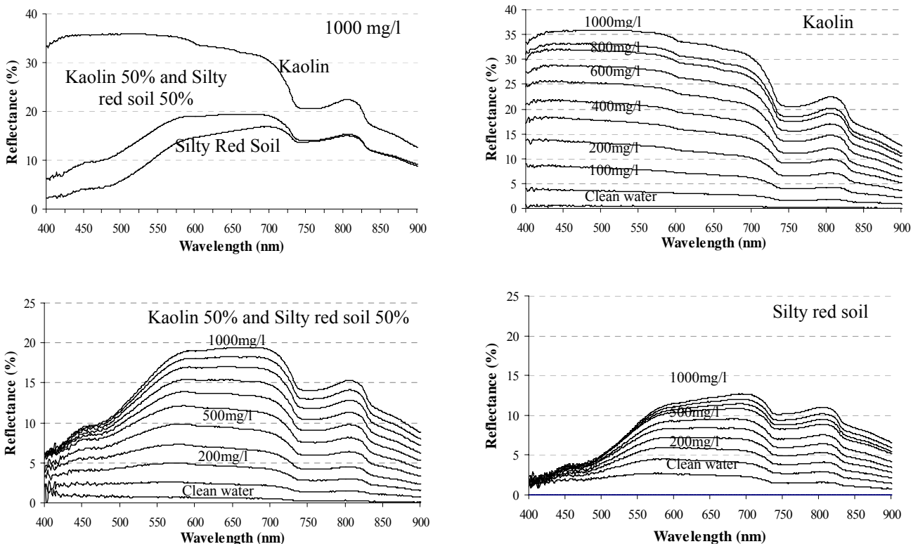
Figure 1: Spectral reflectance of water with different types and concentration of suspended sediments
