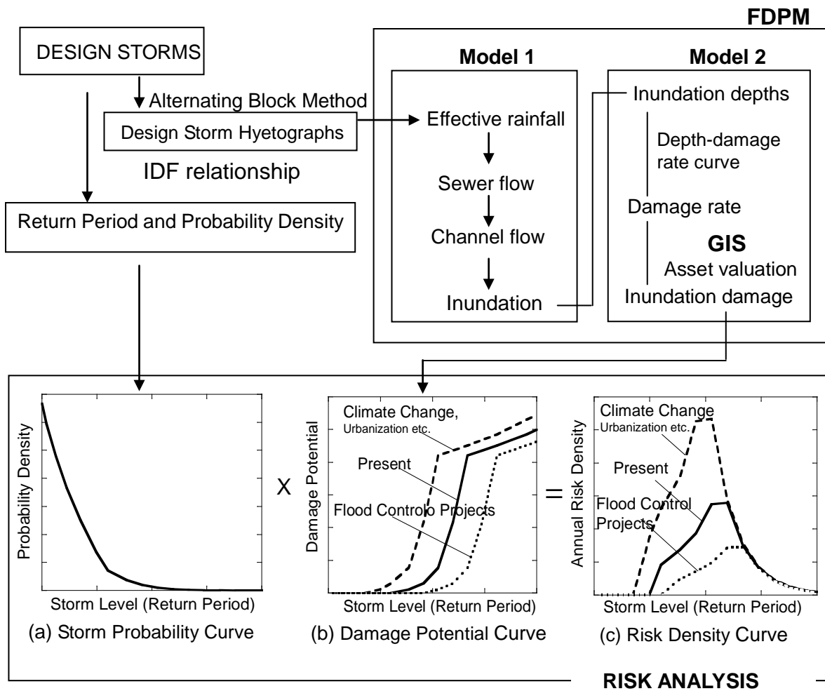
Fig.1 Procedure of flood risk assessment (Design storms, FDP, and Risk Analysis)
