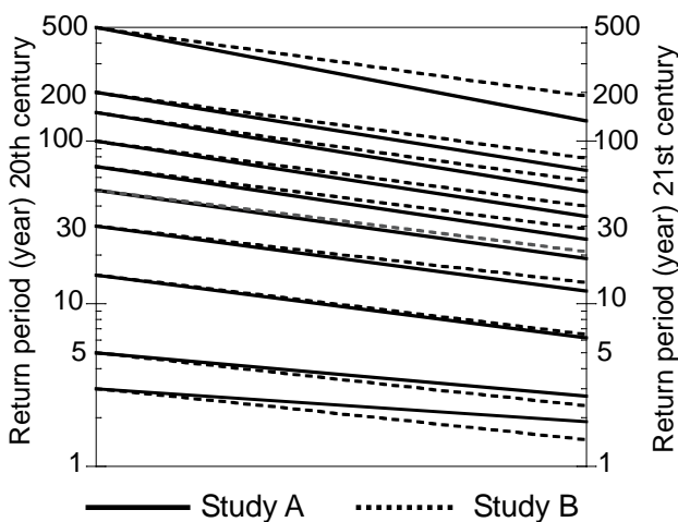
Fig.4 Return periods for 20th and 21st centuries
