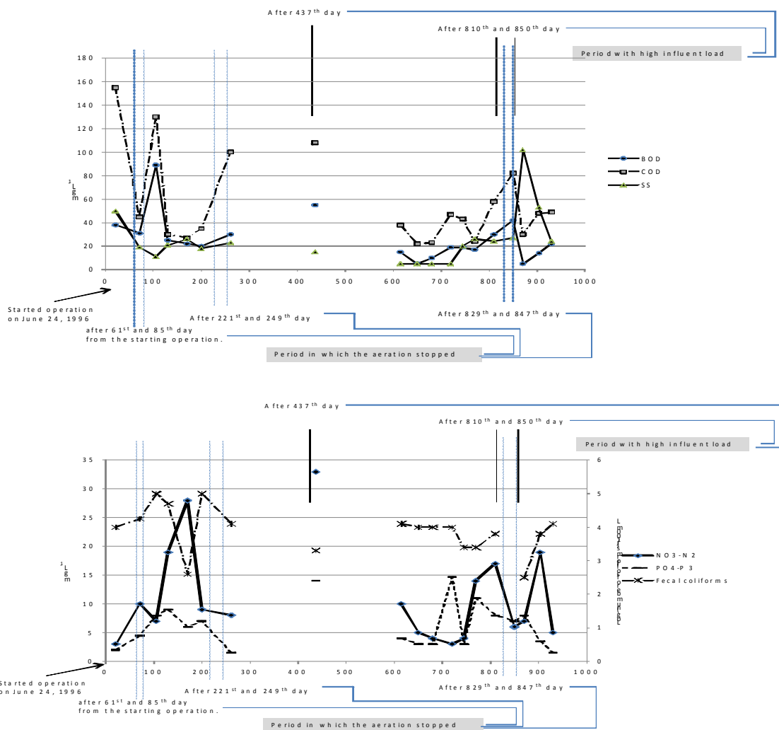
Fig. 3 Results of performance of Johkasou system applied in Cirebon City during the period of 1995-2000 (referred to original source: JICWELS [2000] with some estimates)
