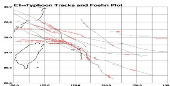
Figure 13 The relationship between the central location of the class 1 typhoon track and the typhoon induced foehn events in the eastern Taiwan.
