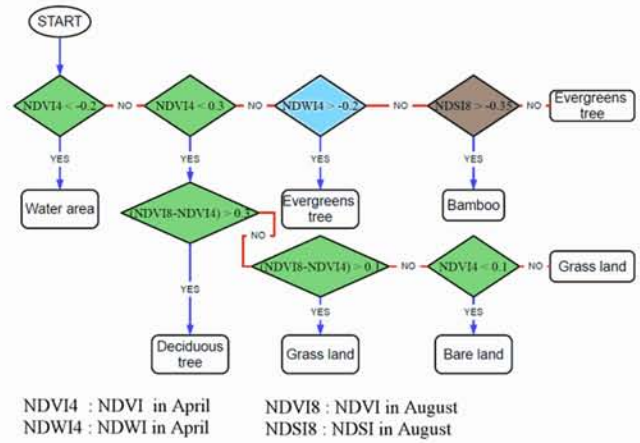
Figure 6.5: Classification algorithm
