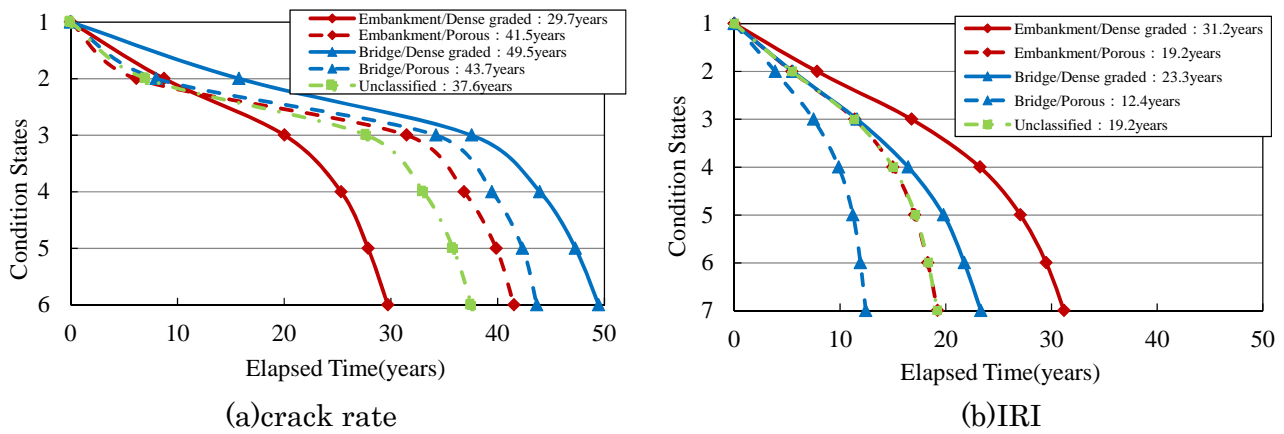
Figure 5 Expected deterioration path according to the evaluation index and surface layer classification (embankment)
