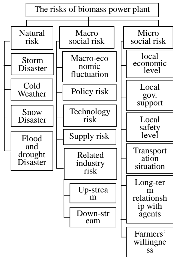
Fig.8 The risks of biomass power plant
