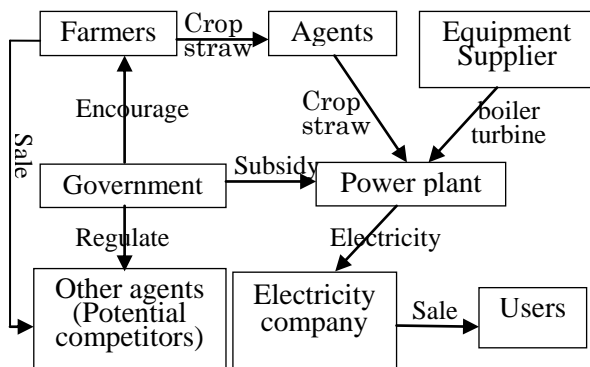
Fig.6 The current stakeholder relationship
