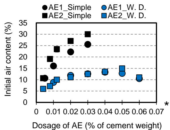
Fig. 5: Effect of water-dividing mixing method (W. D.) on initial air content (*dosage of AE \times 4 in case of AE2)
