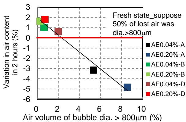
Fig. 18: Relation between stability of air and air volume at fresh state by considering 50% of the lost air was with bubbles diameter larger than 800\mu\text{m}
