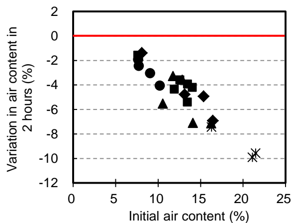
Fig. 2: The loss of air content in 2 hours in fresh mortar with various types of AE (Different shape means different types of AE)
