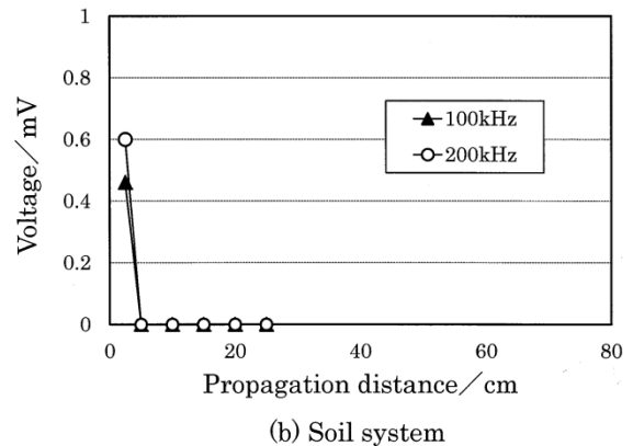
図 8. Propagation distance of ultrasound and voltage generated.
