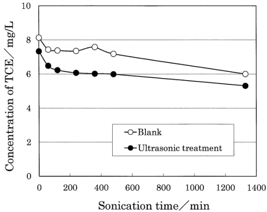
図 7. TCE degradation in TCE contaminated sand with ultrasound.
