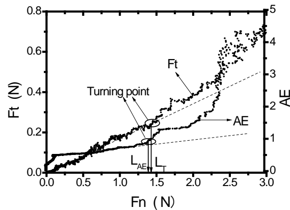
Fig. 3. Variations of the tangential force and AE signal with the normal force (AR).
