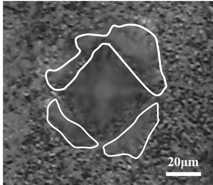
Fig. 6. Micrograph of indentation with 2.94 N.
