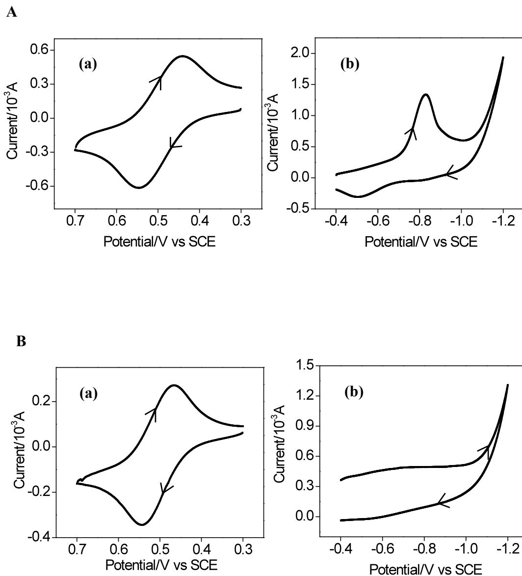
Figure 2.3 Cyclic voltammograms of 0.1wt% iron sulfide samples in suspension at 25°C after electrolytic oxidation at 1.3V for one minute. (A) FeS: (a) ferrous ion, (b) silver sulfide; (B) FeS 2 : (a) ferrous ion, (b) silver sulfide.
