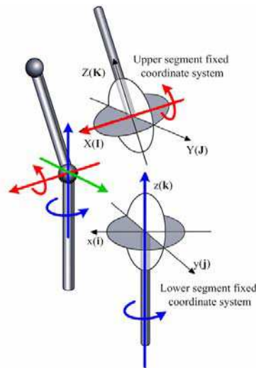
Fig.6-3 Cartesian coordinate system were defined in each rigid body segment. Capitalized letters X, Y, Z denoted the upper segment axes with \mathbf{I}, \mathbf{J}, \mathbf{K} as the respective base vectors, while lower case letters x, y, z denoted the lower segment system axes with \mathbf{i}, \mathbf{j}, \mathbf{k} as their respective base vectors. For both segments, the z axis was positive to the upward, the y axis was positive anteriorly, and the x axis is positive to the right.
