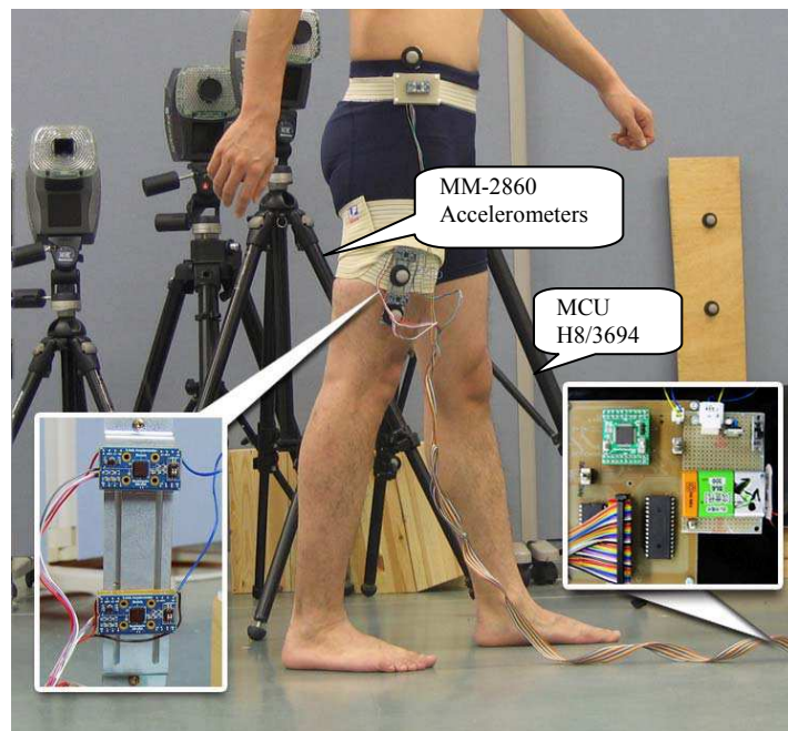
Fig.3-9 Experiment for the lower limb orientation using the developed wearable system
