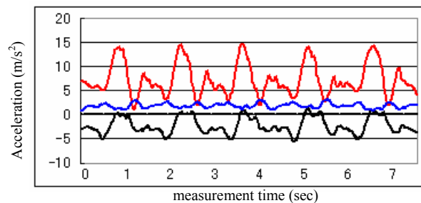
Fig.6-10 One group of accelerations in the knee joint regarded as measured by virtual accelerometers is shown. The virtual accelerations were calculated from the four groups of accelerations measured by the four physical accelerometers on the thigh and shank. The red line is the acceleration about y axis, black line is the acceleration about x axis, blue line is the acceleration about z axis in the sensor coordinate system
