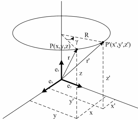
Fig.1- 6. Rotation about the z-axis of the coordinate system.
