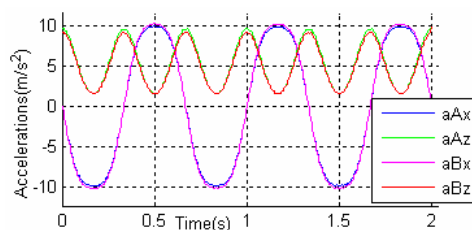
a. Given accelerations of each axis in local frame on positions A and B
