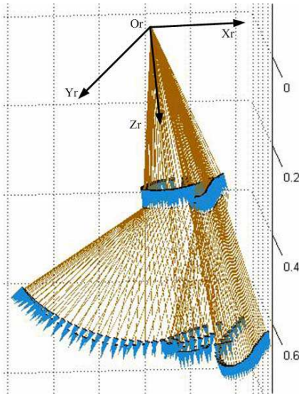
Fig.6-14 One gait circle shown by continuous stick figures for visual and quantitative confirmation of the human gait posture. The blue arrows represent the knee joint and ankle joint.
