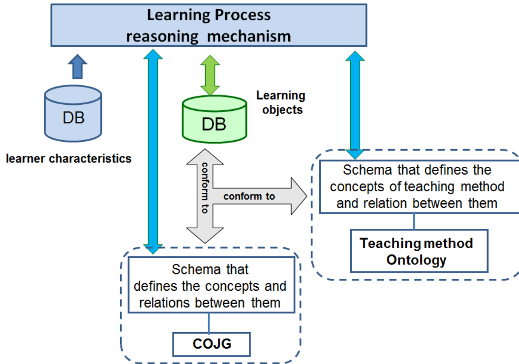
Fig. 3.1. The system framework of CLLSS.
