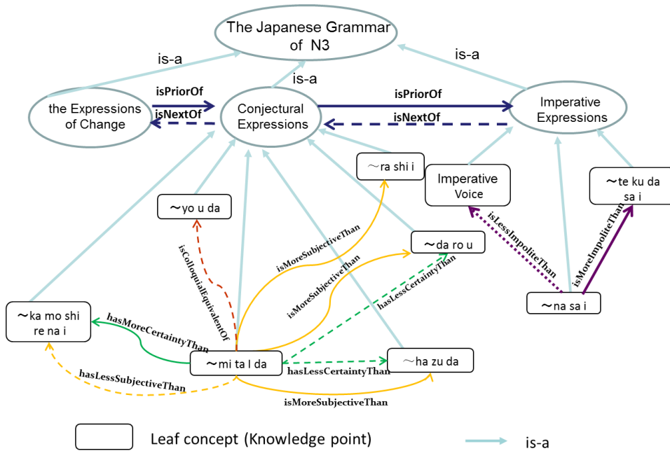
Fig. 2.5. Another example of relation schema of COJG
