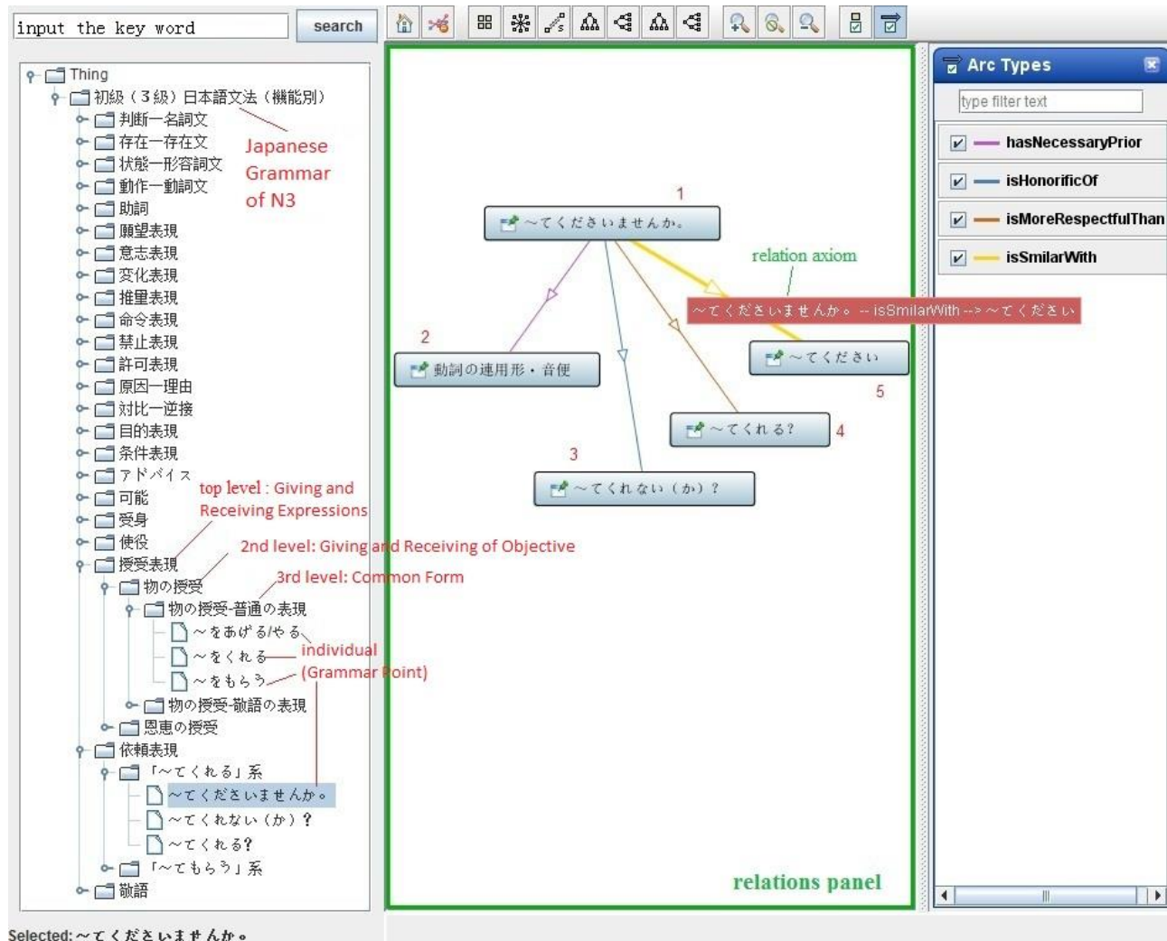
Fig. 3.3. Common view of CLSS (1.0) for both instructors and learners.
