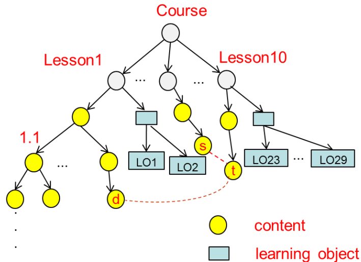
Fig. 2.1. An example of the tree structure in Moodle system.
