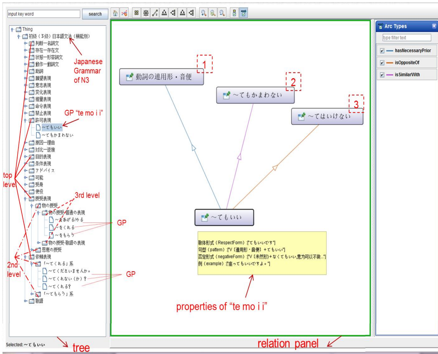
Fig. 4.1. The common view of CLLSS 2.0 for both instructors and learners.
