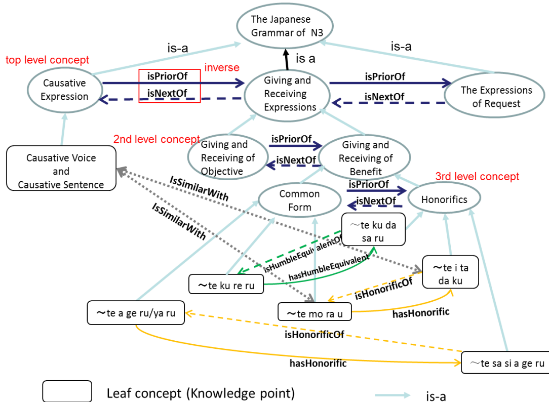
Fig. 2.2. A partial relation schema of COJG
