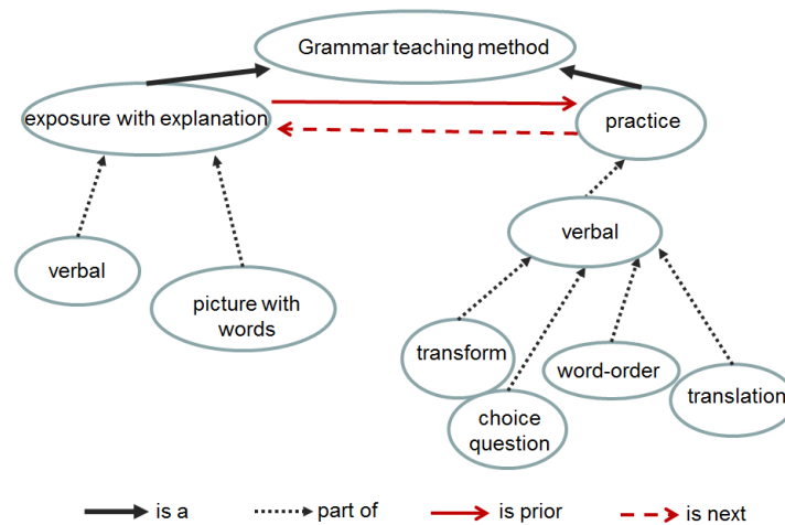
Fig. 3.2. A partial structure of grammar teaching method ontology.
