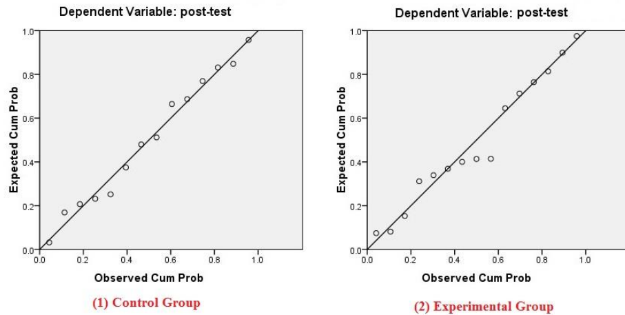
Fig. 3.6. Normal P-P Plots of Regression Standardized Residuals
