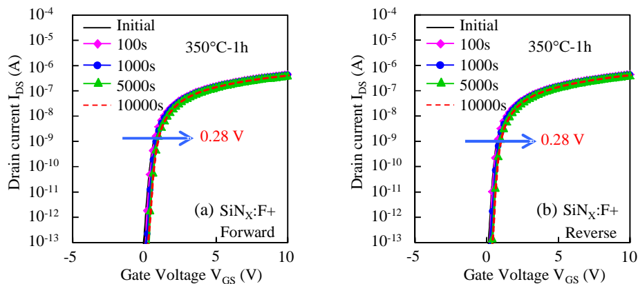
Fig. 5.4 Change in transfer characteristics during NBIS ( \lambda=460 nm) for the IGZO TFTs with \text{SiN}_x\text{:F+} passivation.
