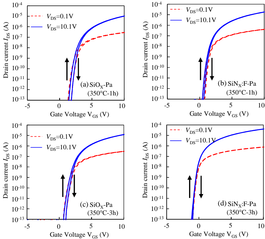
Fig. 4.6 Transfer characteristics of the TFTs with \text{SiO}_x or \text{SiN}_x\text{:F} passivation after annealing in \text{N}_2 ambient at 350 °C for different annealing times. Annealing times are (a) (b) 1h and (c) (d) 3h for the \text{SiO}_x and \text{SiN}_x\text{:F} passivations, respectively.
