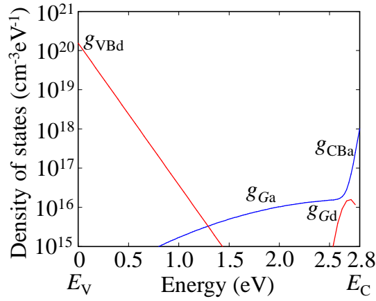
Fig. 3.7 Bulk DOS of a-ITZO model used in the device simulation.
