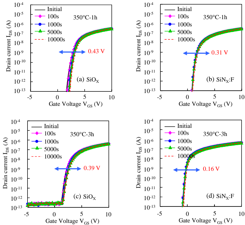
Fig. 4.15 Change in transfer characteristics during NBS without light for the IGZO TFTs with (a) \text{SiO}_X and (b) \text{SiN}_X:\text{F} passivations after \text{N}_2 annealing at 350^\circ\text{C} for 1h; (c) \text{SiO}_X and (d) \text{SiN}_X:\text{F} passivations after \text{N}_2 annealing at 350^\circ\text{C} for 3h.
