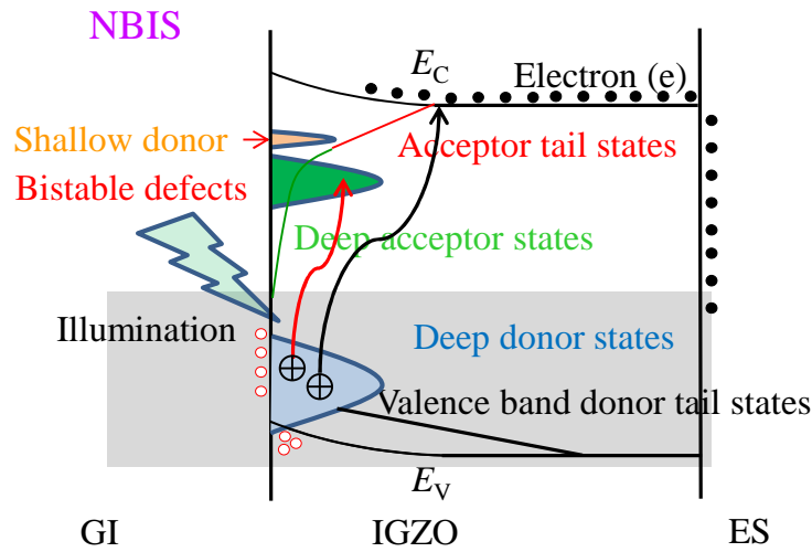
Fig. 4.19 Degradation mechanism of IGZO TFTs with \text{SiO}_x or \text{SiN}_x\text{:F} passivation under NBIS after \text{N}_2 annealing at 350^\circ\text{C} for 1h.
