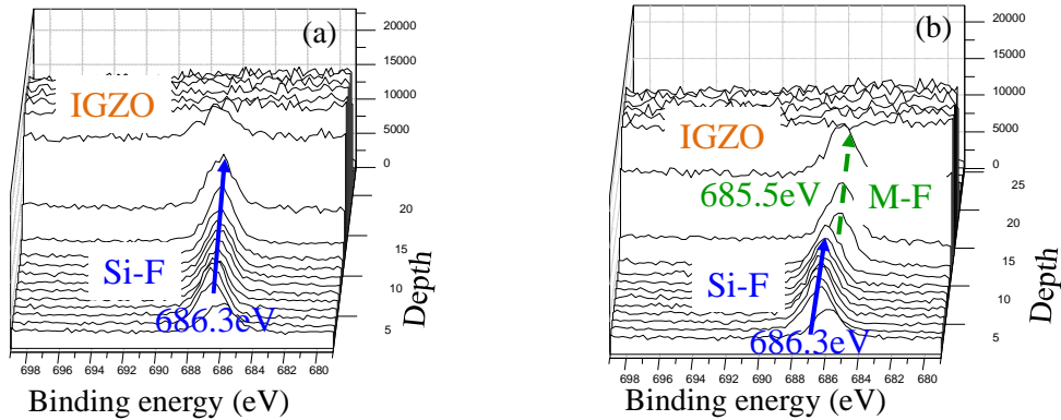
Fig. 4.4 F substituted M-O to M-F (a) as fabrication (b) after N 2 annealing at 300 °C.
