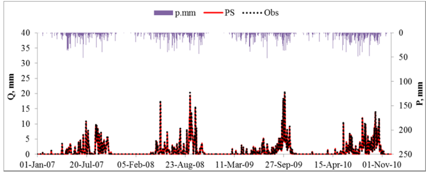
(b) Runoff calculated at PS basin
