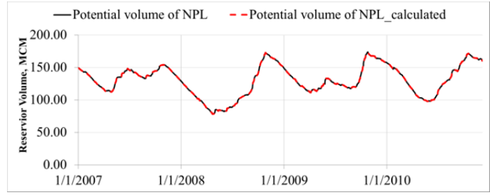
(b) Reservoir volumes of calculated and recorded data at NPL
