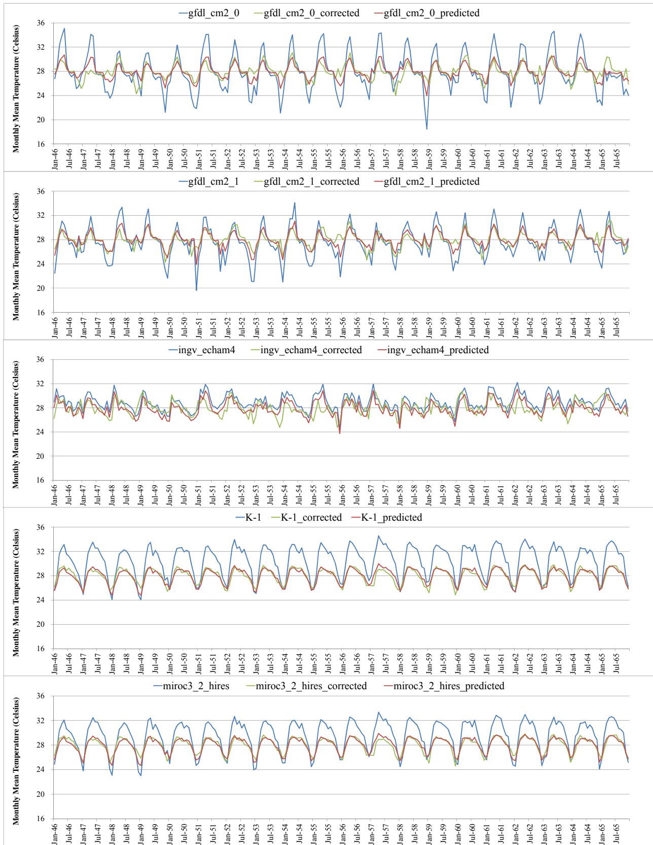
Fig. 7-5 Corrected mean temperature parameter in future year (2046-2065)
