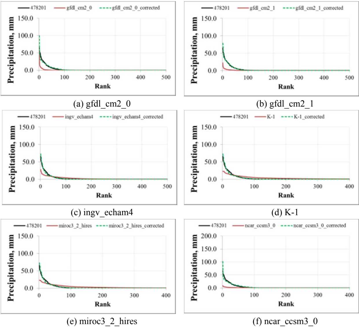
Fig. 5-13 The distribution of precipitation data from GCMs and corrected precipitation data of six GCMs compared to distribution of precipitation data at rain gauge station No.478201 in dry season (For example)
