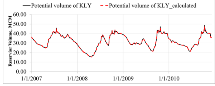
(c) Reservoir volumes of calculated and recorded data at KLY
