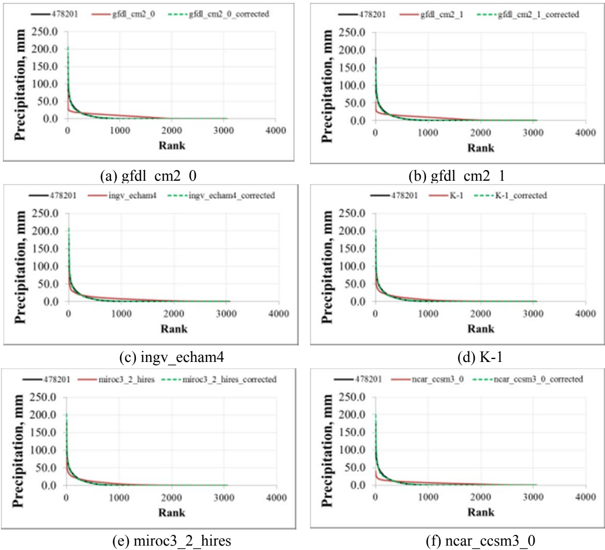
Fig. 5-14 The distribution of precipitation data from GCMs and corrected precipitation data of six GCMs compared to distribution of precipitation data at rain gauge station No.478201 in first rainy season (For example)
