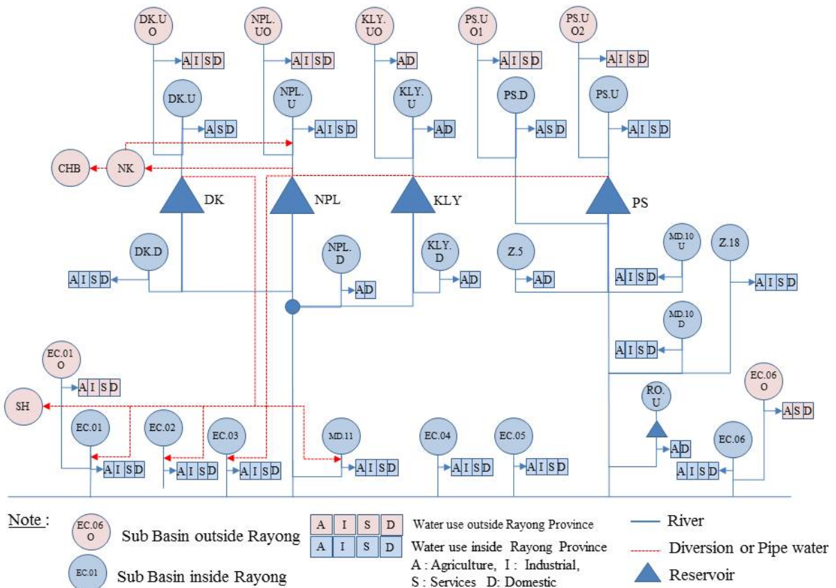
Fig. 6-9 Network Tank model was developed with Rayong water user diagram
