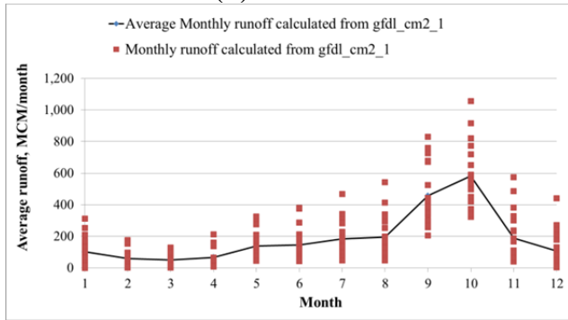
(c) gfdl_cm2_1
