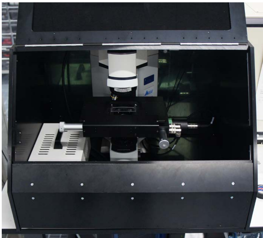
Figure 3.6. Micro-Raman spectrometer HORIBA JOBIN YVON HR-800.
