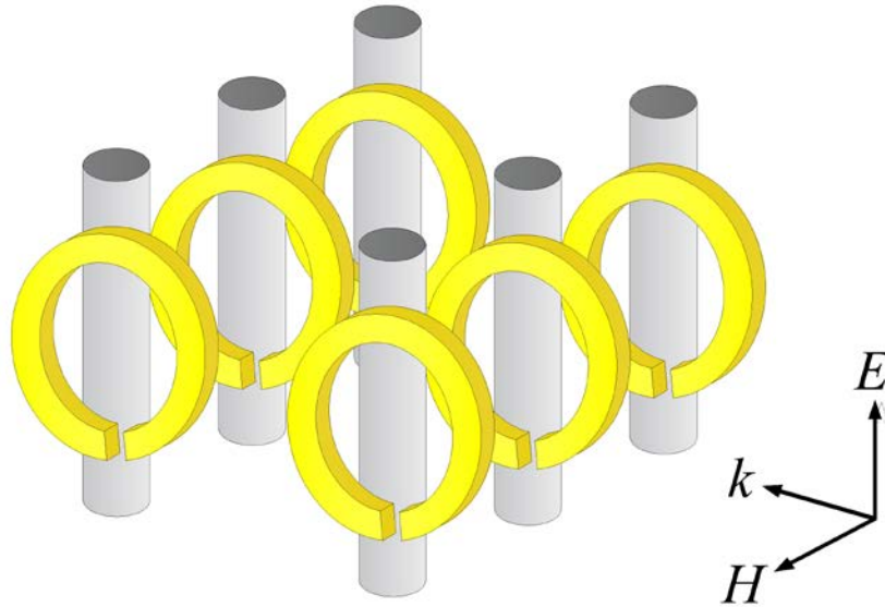
Figure 2.16. Example of structure composed of thin metal wires and split rings, used for generation of electromagnetic resonance in metamaterials.
