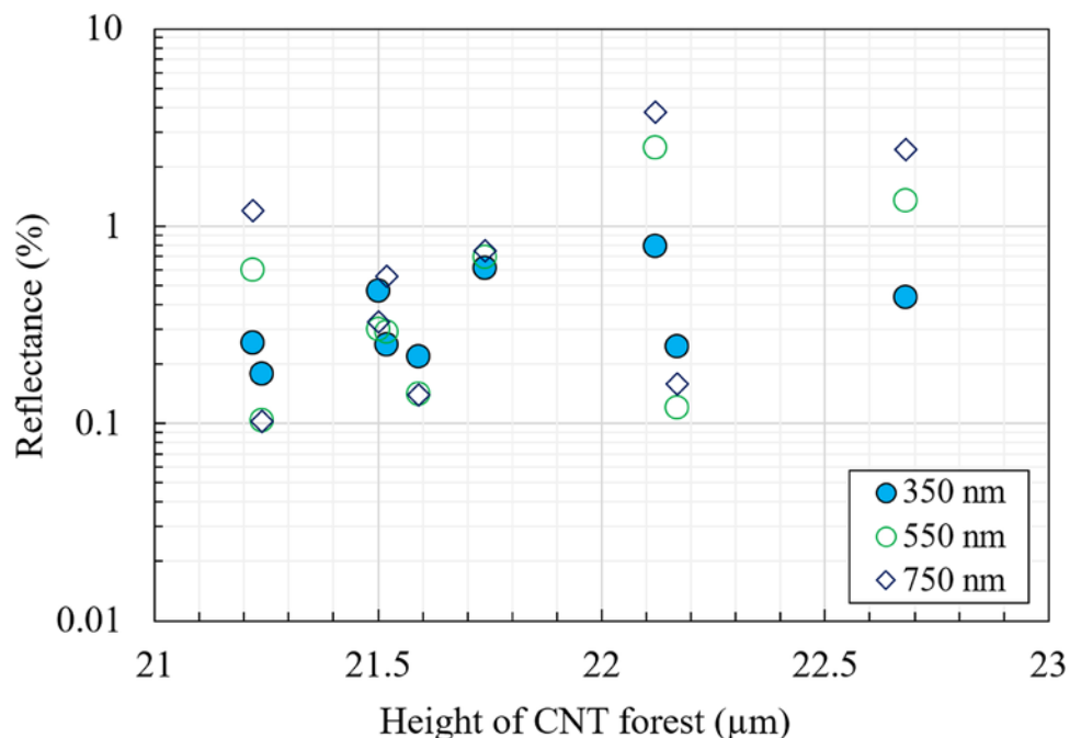
Figure 5.2. Height of CNTs vs total optical reflectance for 350 nm, 550 nm, and 750 nm [submitted to Journal of Materials Science].
