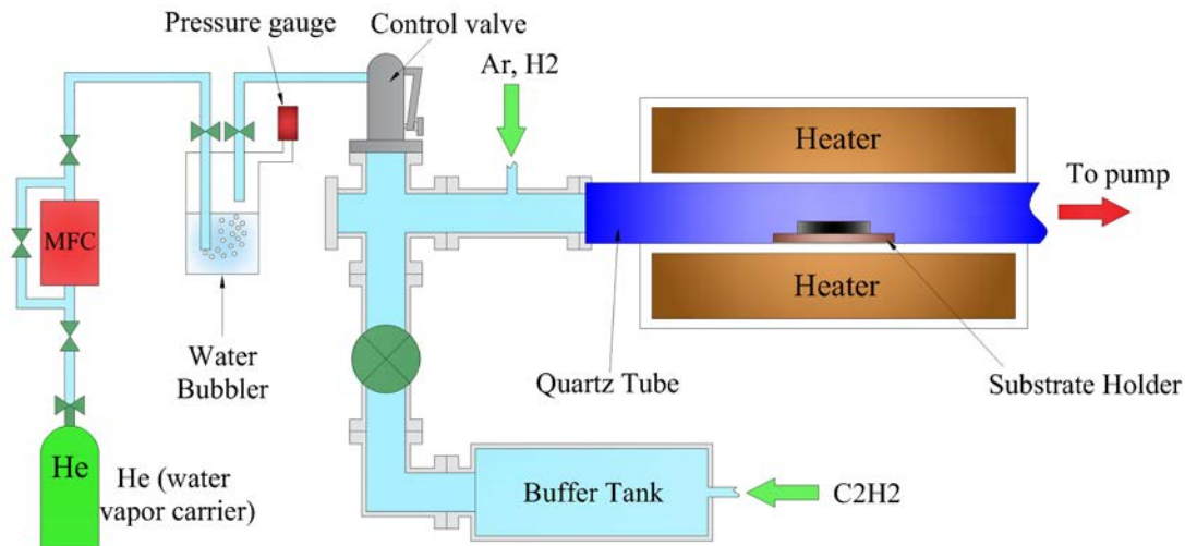
Figure 6.1. The schematic of modifications of CVD chamber for water-assisted CNT growth [183].
