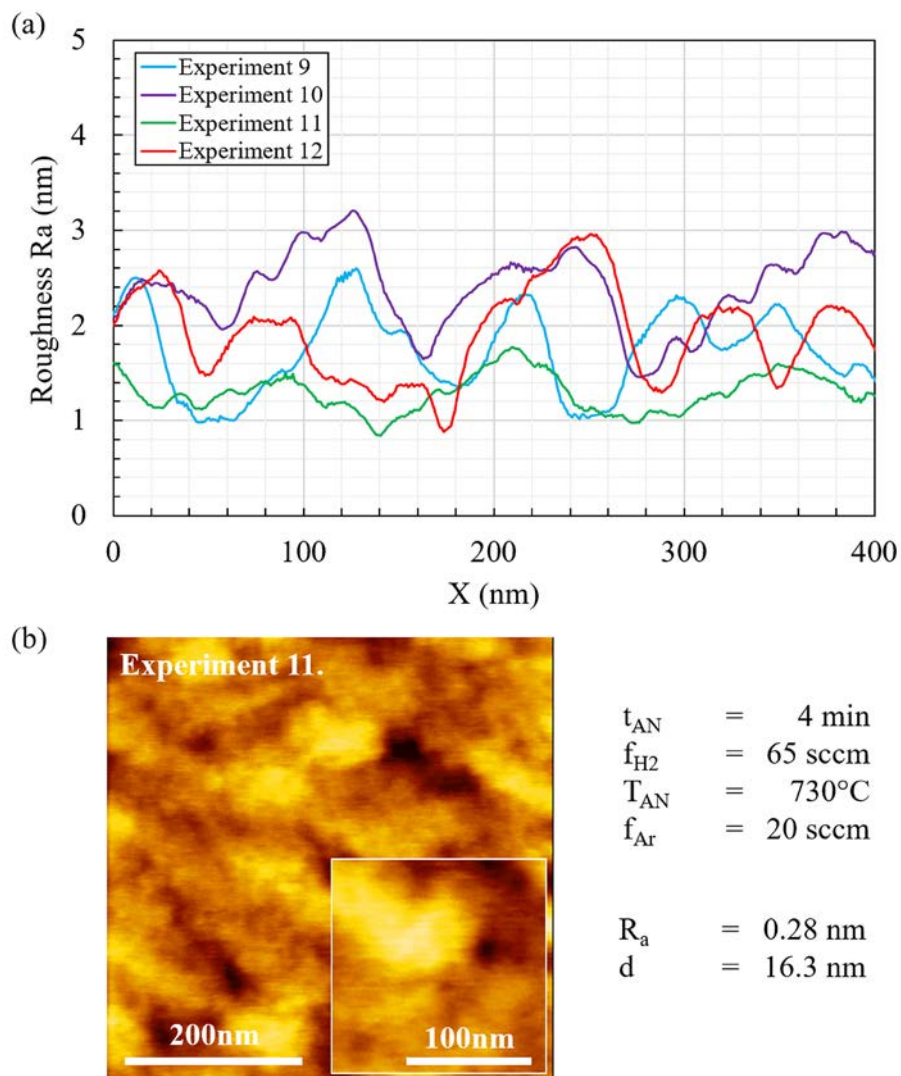
Figure 4.5. (a) AFM line profiles of Fe catalyst particles after annealing process for the Taguchi experiments 9-12, (b) AFM scan of surface of experiment 11, with process parameters and results of measurements. Fixed parameter in Exp. 9-12 was annealing time of 4 min [161].
