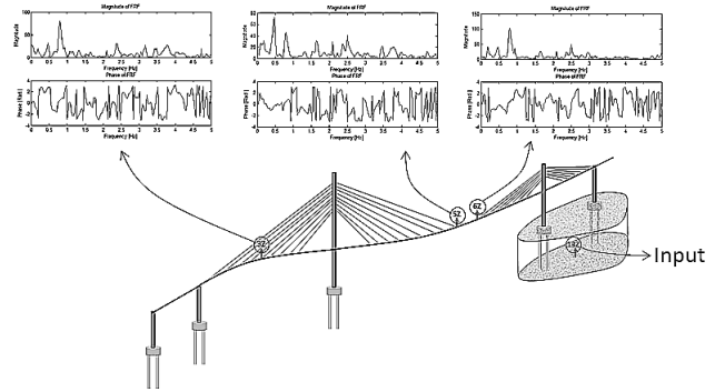
Figure 14 FRF Z-Direction of earthquake II
