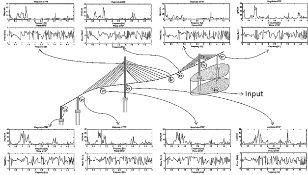
Figure 10 FRF Y-Direction of earthquake I
