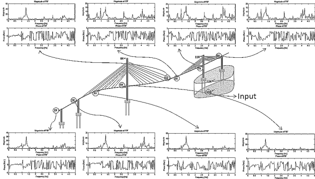
Figure 9 FRF X-Direction of earthquake I
