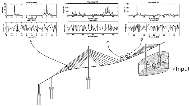
Figure 11 FRF Z-Direction of earthquake I
