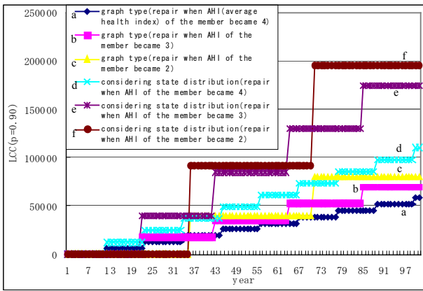
Fig.10 LCC (p=0.90)
