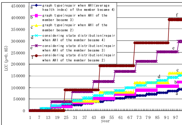
Fig.11 LCC (p=0.85)
