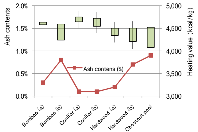
Figure 2. Comparison of heating value and ash contents in different raw materials
