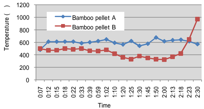
Figure 4. Changes in temperature in the furnace
