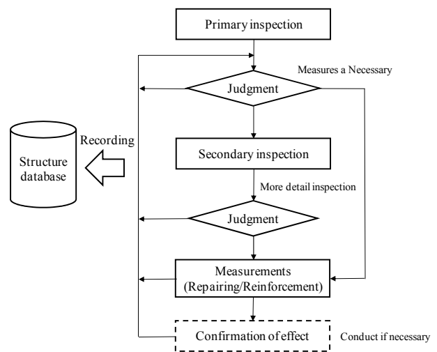
Figure 3 Maintenance flow of power cable tunnel
